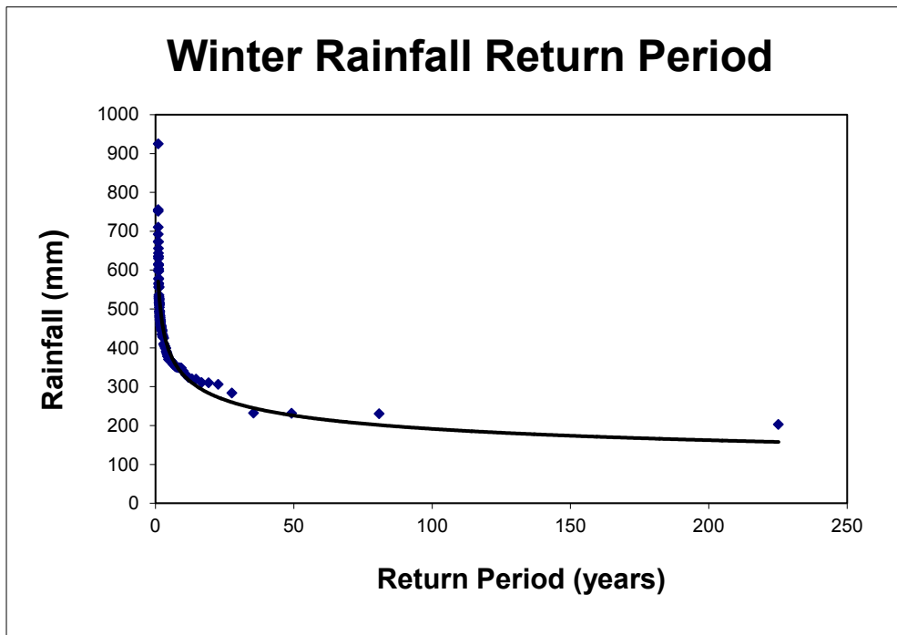
Figure 6: Return Period of Winter Rainfall
