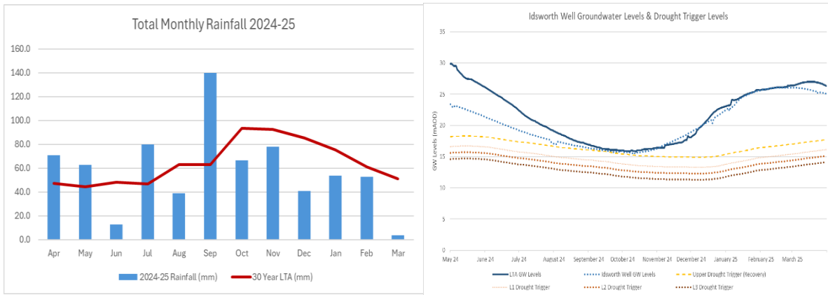
Figure 2 Monthly rainfall, groundwater levels and Drought Trigger Levels in 2024-25
