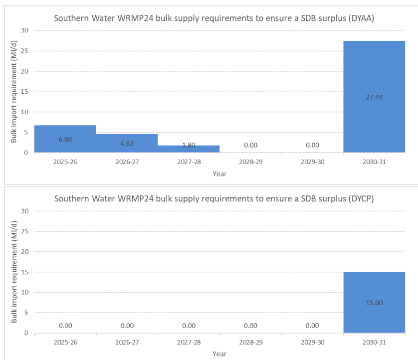
Figure D: Southern Water WRMP24 minimum bulk supply requirements to ensure a SDB surplus
