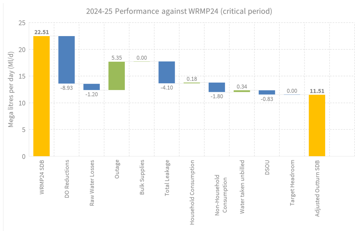
Figure 10: 2024-25 Performance compared against updated WRMP24 (Critical Period)
