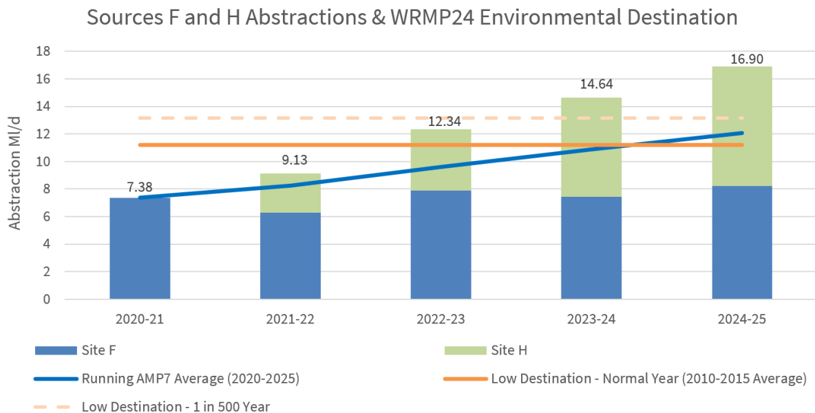
Figure 12: Sources F and H abstractions during AMP7 compared to Environmental Destination scenarios
