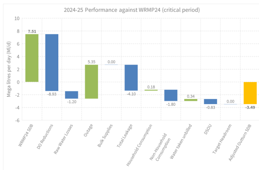
Figure B: 2024-25 Performance compared against WRMP24 (Critical Period)
