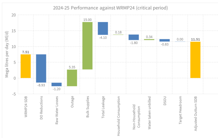
Figure B: 2024-25 Performance compared against WRMP24 (Critical Period)
